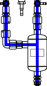
Check Valve as a Zone Separator
