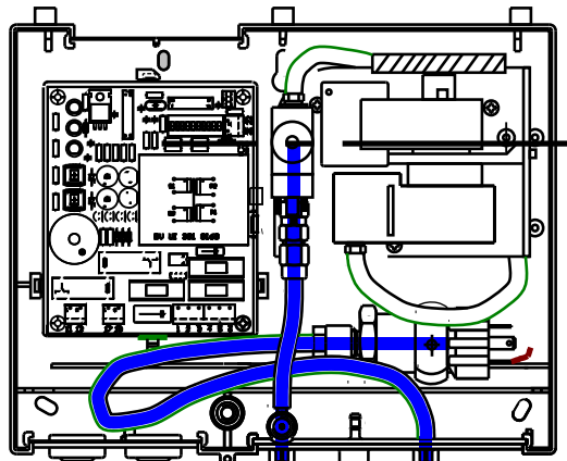
Solenoid Valve as a Zone Separator
