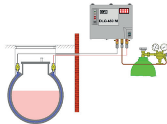
Installation scheme
